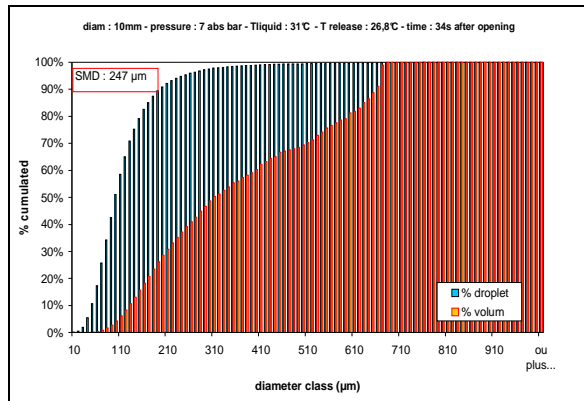
Figure 7. Droplet size distribution data for INERIS experiment 2 (10 mm orifice, 6 barg, 26.8C)
