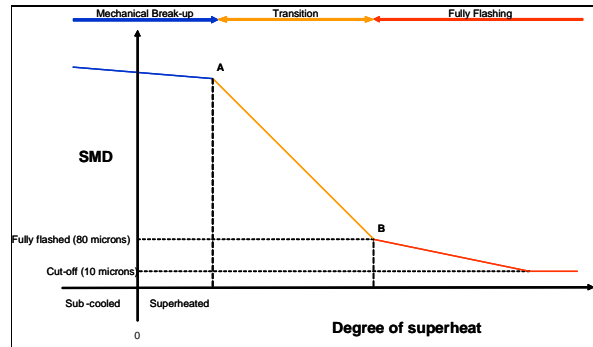
Figure 3. Tri-linear curve for Sauter Mean Diameter (SMD) as function of superheat
