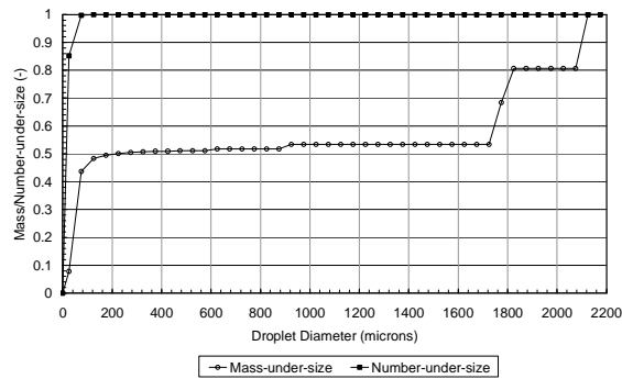
(a) flashing jet (2 mm, L/d_o=0.5 , P=10 barg)
