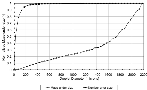
(b) sub-cooled jet (2 mm, L/d_o=0.5 , P=10 barg)
