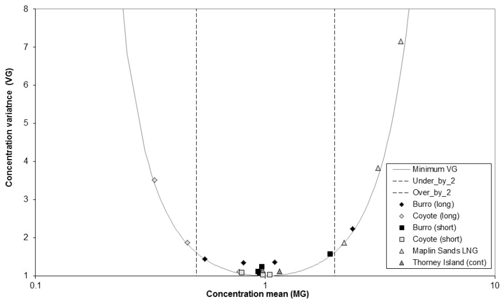
Figure 2: Plot of MG and VG values (arcwise concentrations) for individual field experiments
