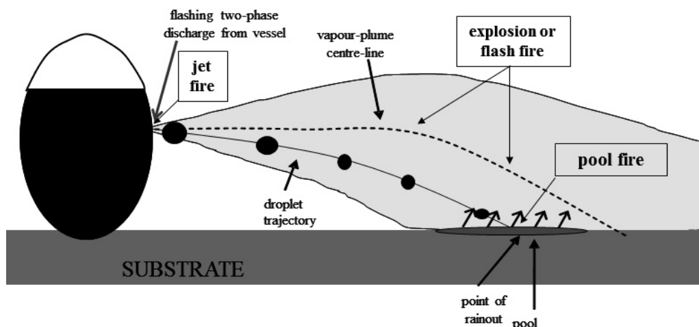
Figure 1: Continuous two-phase release of flammable material with rainout
